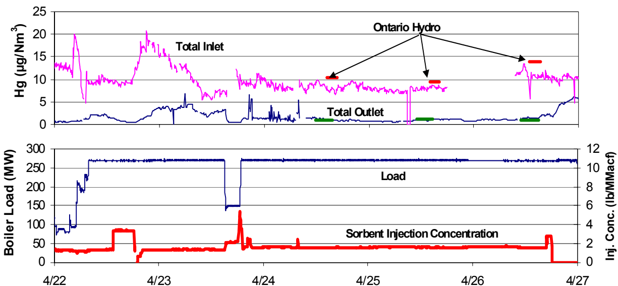
Figure 3. Inlet and Outlet COHPAC Mercury Concentrations, Boiler Load and ACI, Plant Gaston, 2001.
