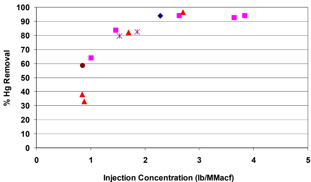
Figure 2. Mercury Removal with Activated Carbon Injected Upstream of COHPAC at Alabama Power Plant Gaston, Spring 2001.
